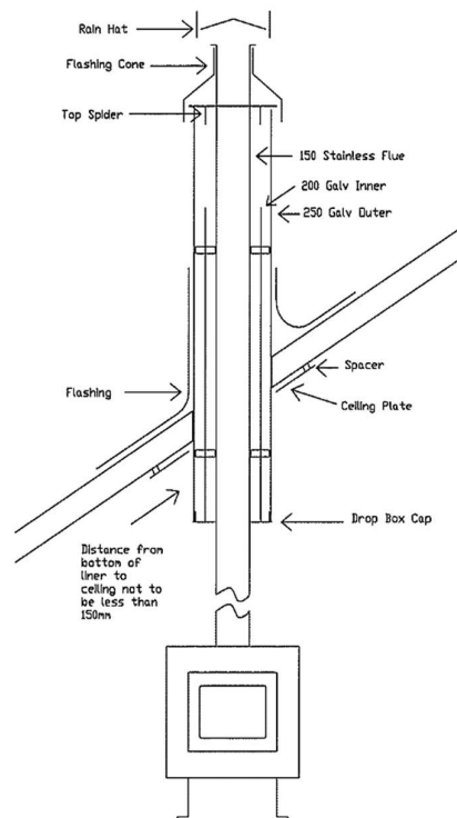
Sloping Ceiling Diagram
