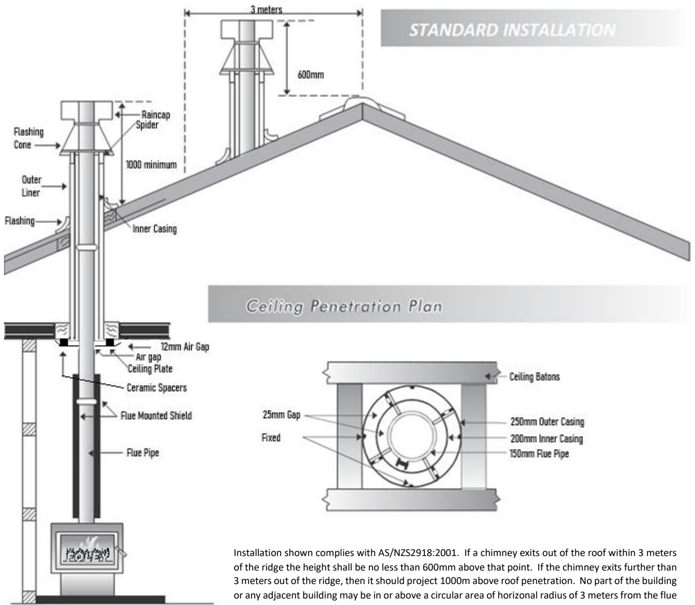
Flat Ceiling Diagram
